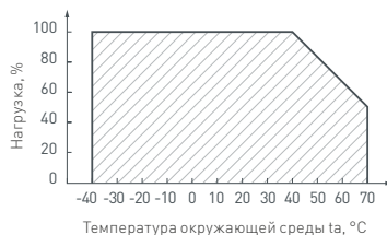
ARPV-12100-SLIM-PFC-B, ARPV-24100-SLIM-PFC-B
